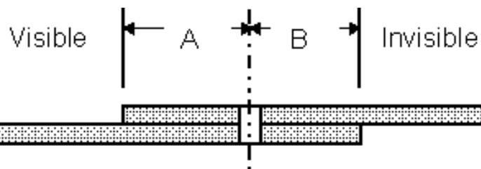
Non-flush Rivets, Plain Holes
