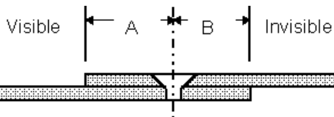
25-19 Rivet, Special Flush Countersunk Hole
